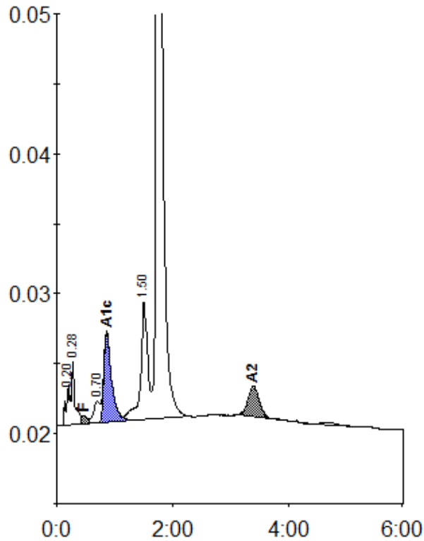
Peak table - ID: 11468858
