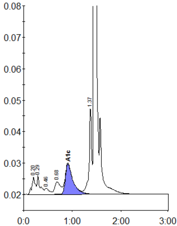
Peak table - ID: 11136055
