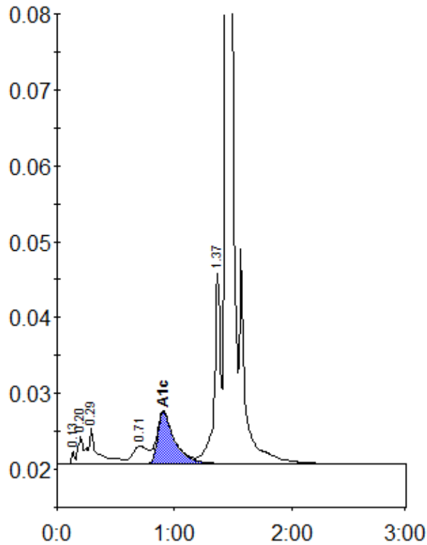
Peak table - ID: 11539904
