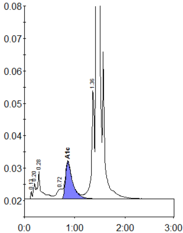
Peak table - ID: 11183193
