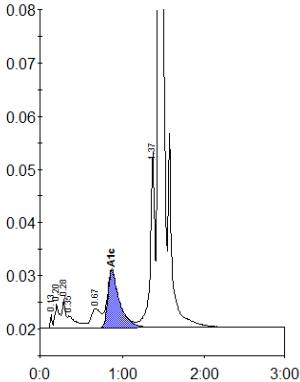
Peak table - ID: 11561681
