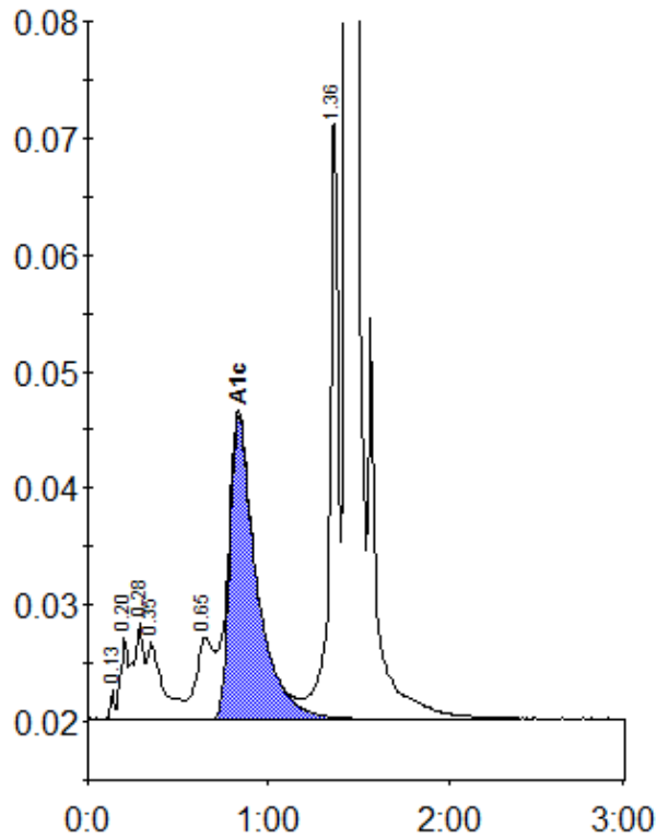
Peak table - ID: 11609343
