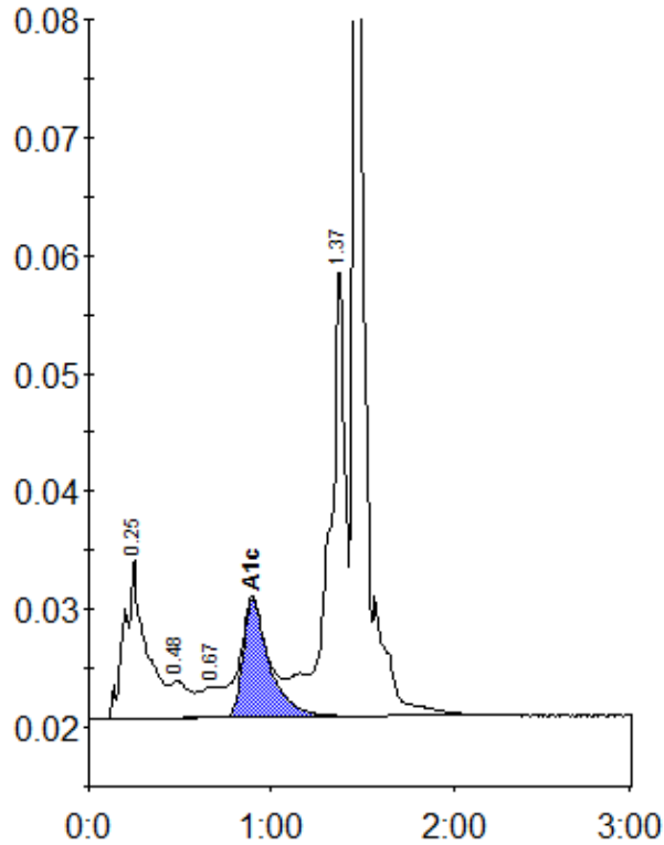
Peak table - ID: 11461024
