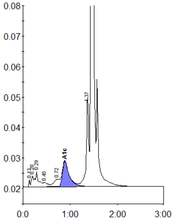
Peak table - ID: 11183255
