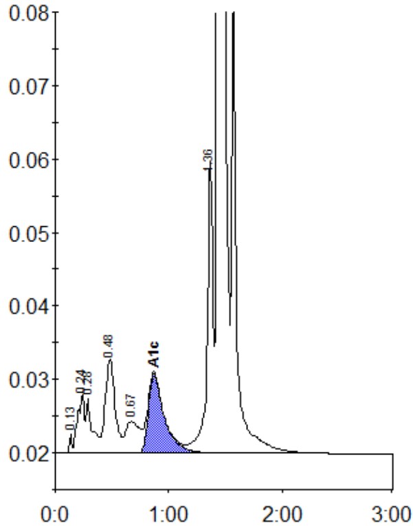
Peak table - ID: 11398002
