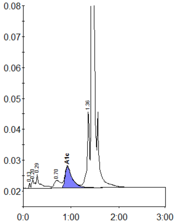
Peak table - ID: 11569445
