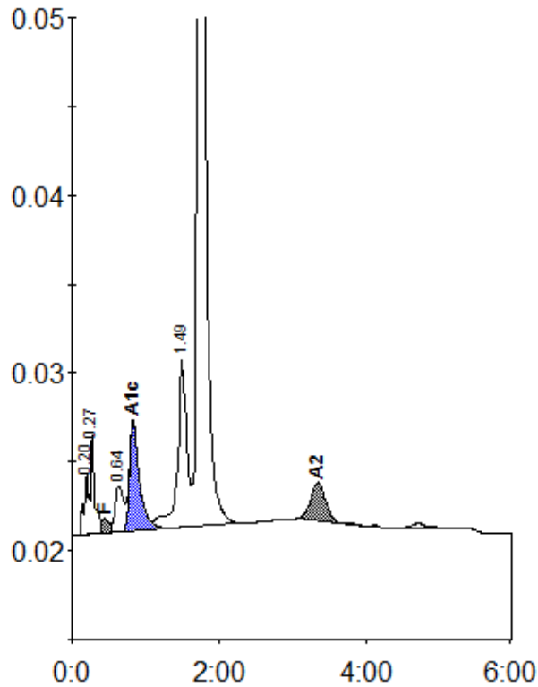
Peak table - ID: 11579300
