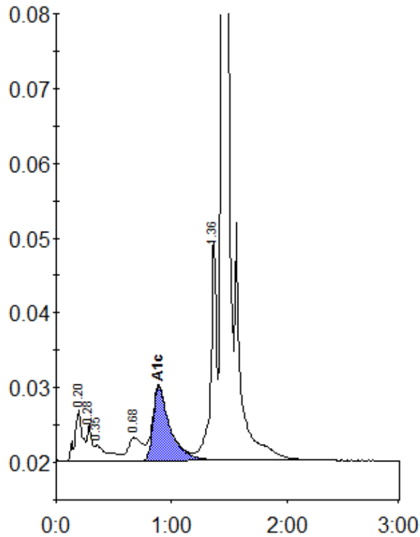
Peak table - ID: 11570729
