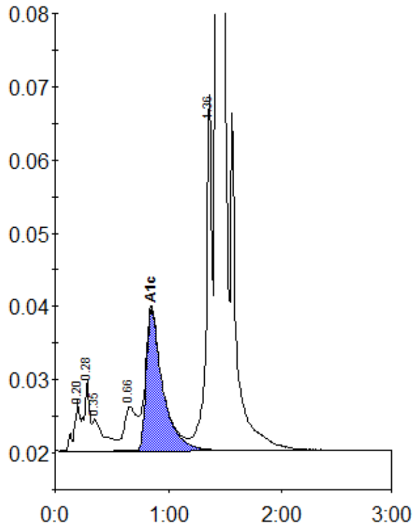
Peak table - ID: 11601257
