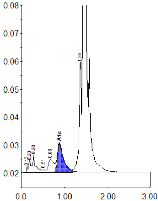
Peak table - ID: 11628947
