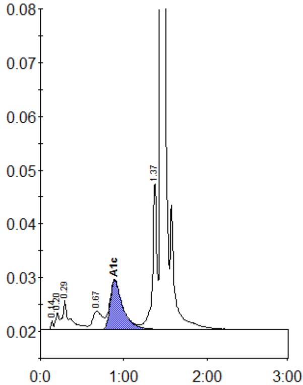
Peak table - ID: 11408719
