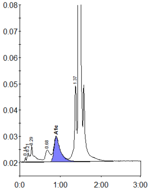
Peak table - ID: 11445665
