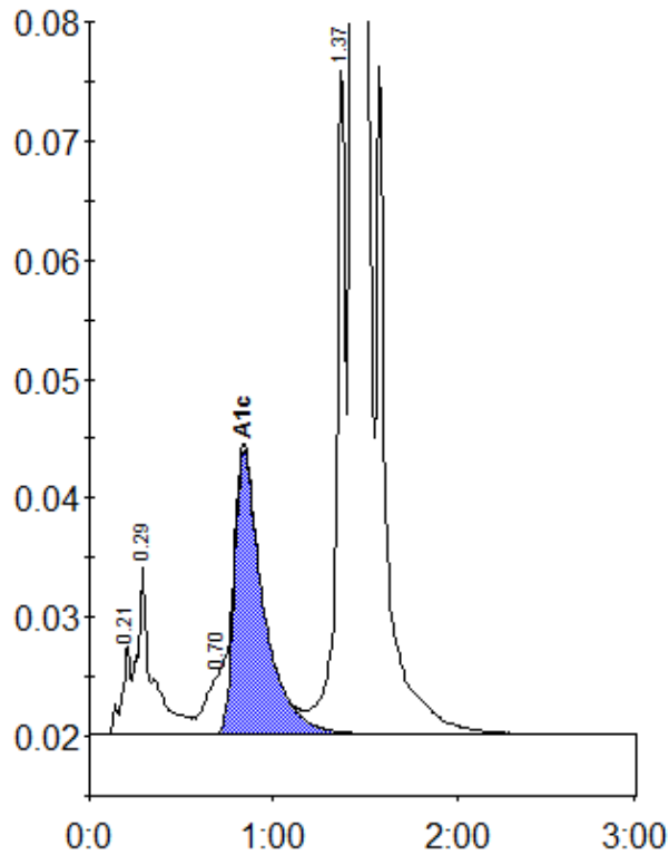
Peak table - ID: 11600273
