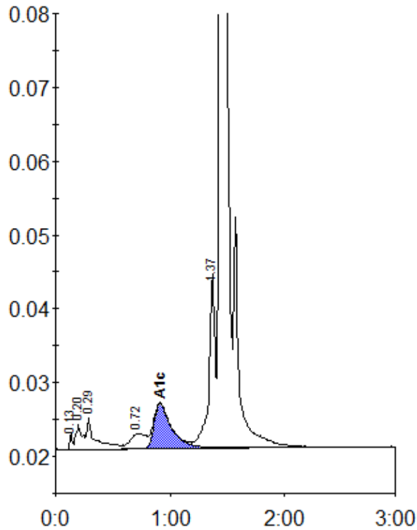
Peak table - ID: 11136348
