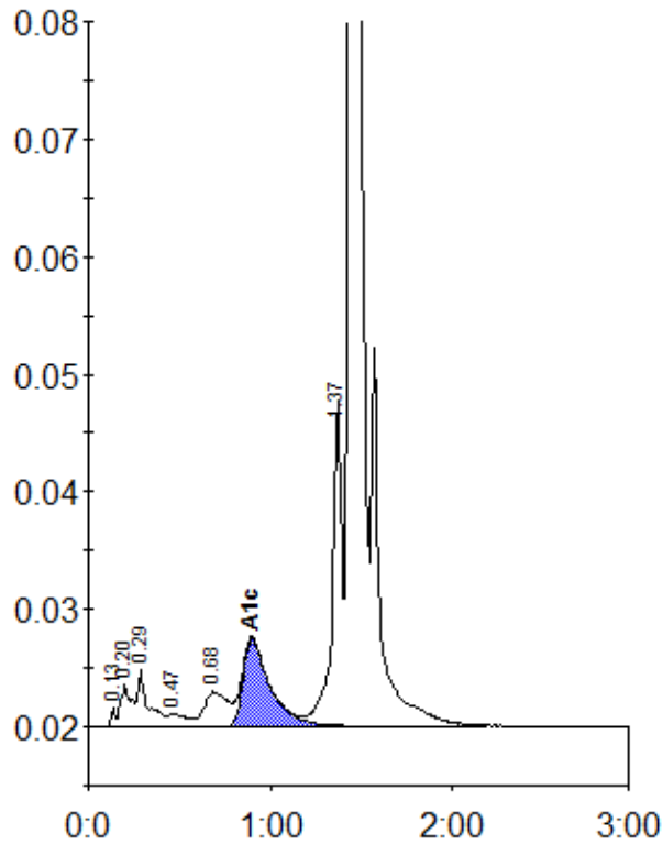
Peak table - ID: 11408671
