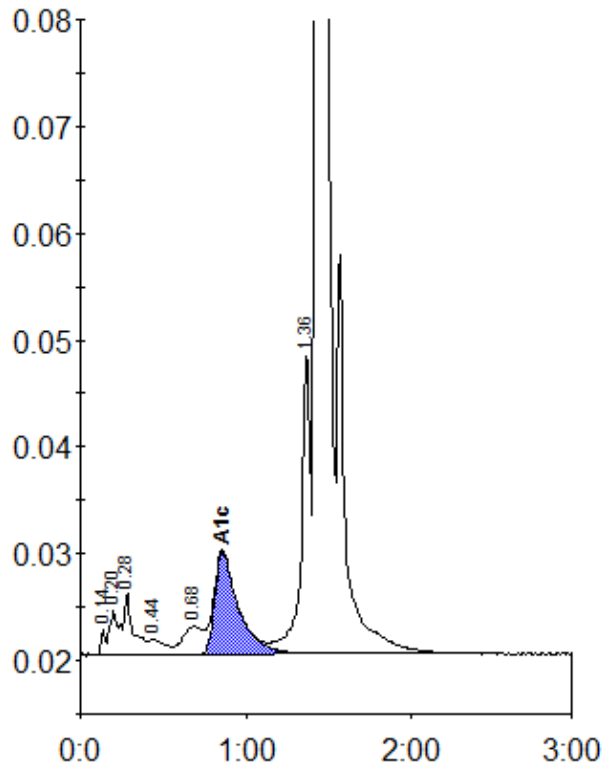
Peak table - ID: 11604035
