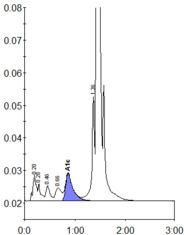
Peak table - ID: 11621753
