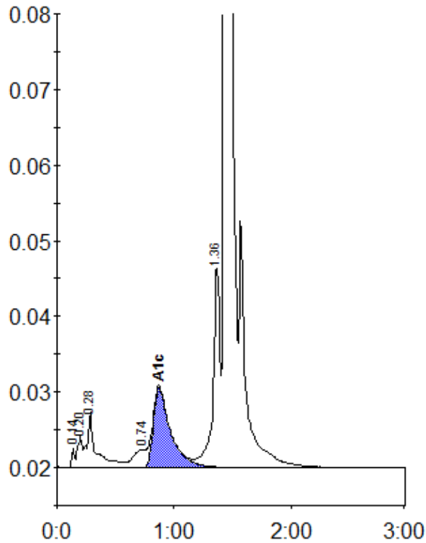
Peak table - ID: 11183674
