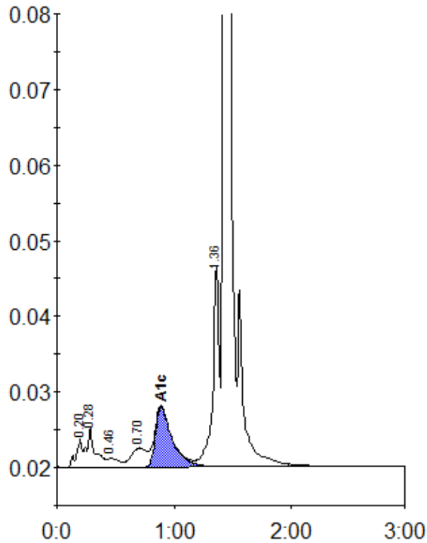
Peak table - ID: 11196040
