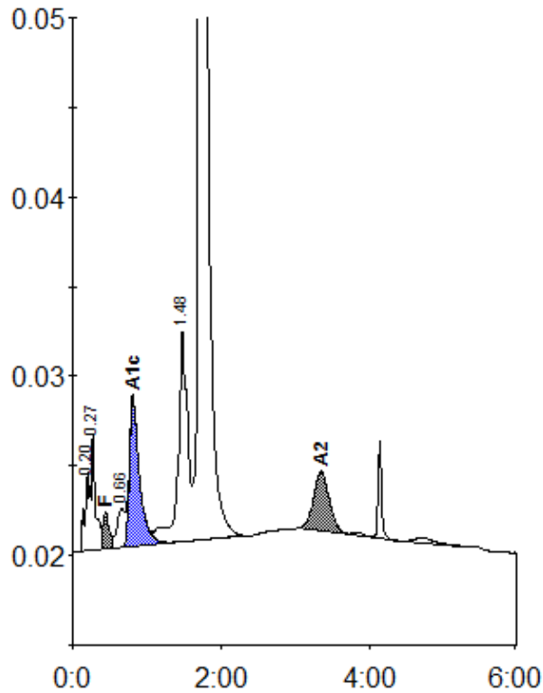
Peak table - ID: 11247798
