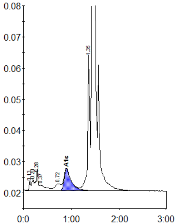
Peak table - ID: 11600476
