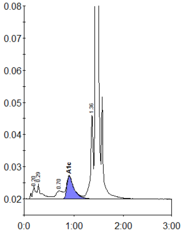
Peak table - ID: 11263519
