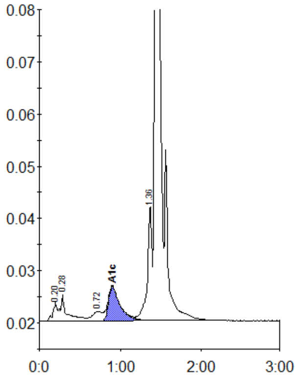
Peak table - ID: 11183813
