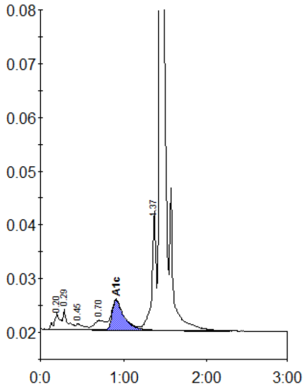
Peak table - ID: 11461758
