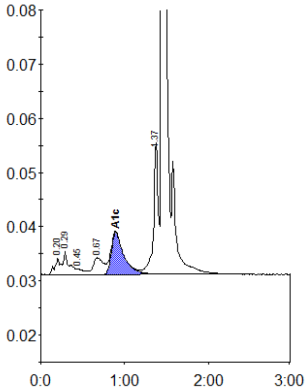
Peak table - ID: 11450228
