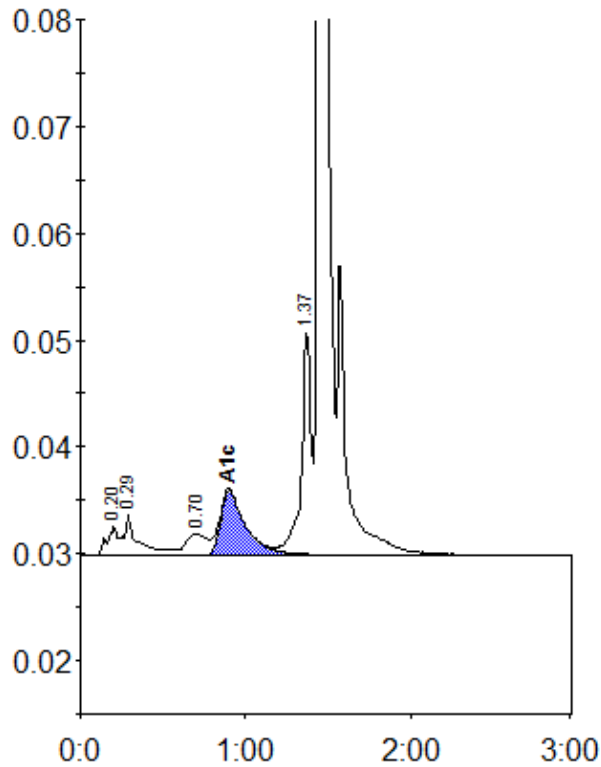
Peak table - ID: 11460186
