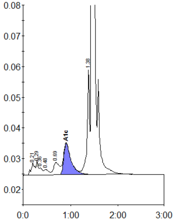
Peak table - ID: 11447558
