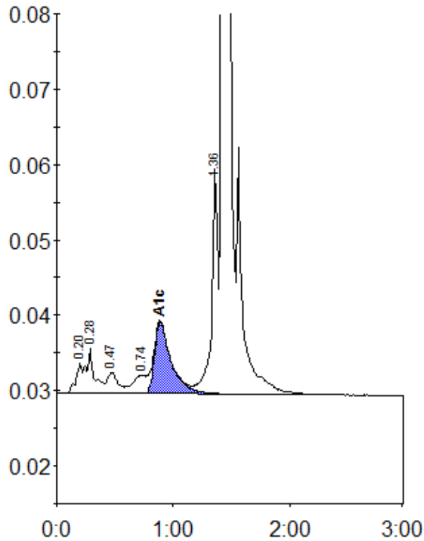
Peak table - ID: 10887401
