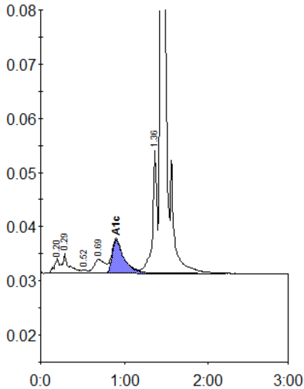
Peak table - ID: 11447221
