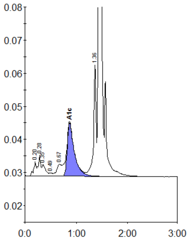
Peak table - ID: 11444814
