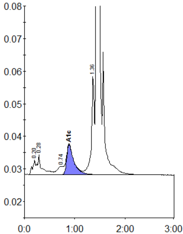
Peak table - ID: 11187082
