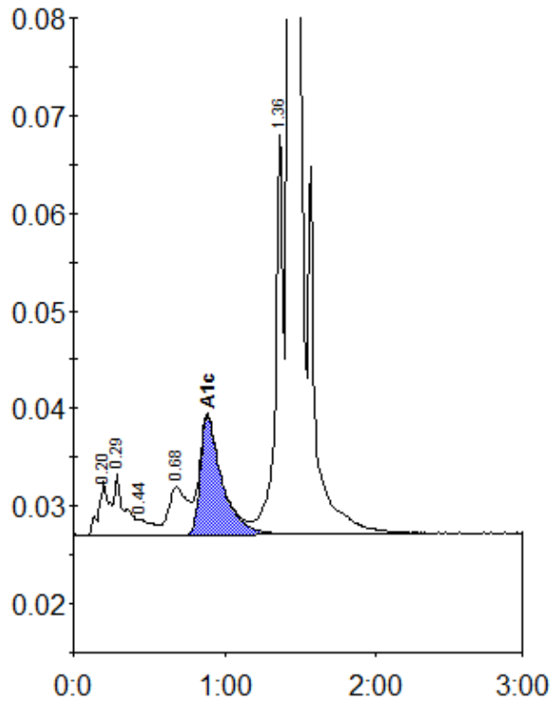
Peak table - ID: 11400496
