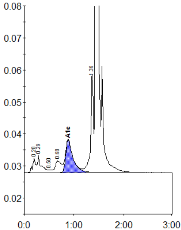
Peak table - ID: 11298013
