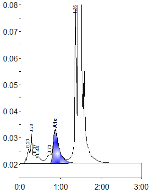
Peak table - ID: 11268099
