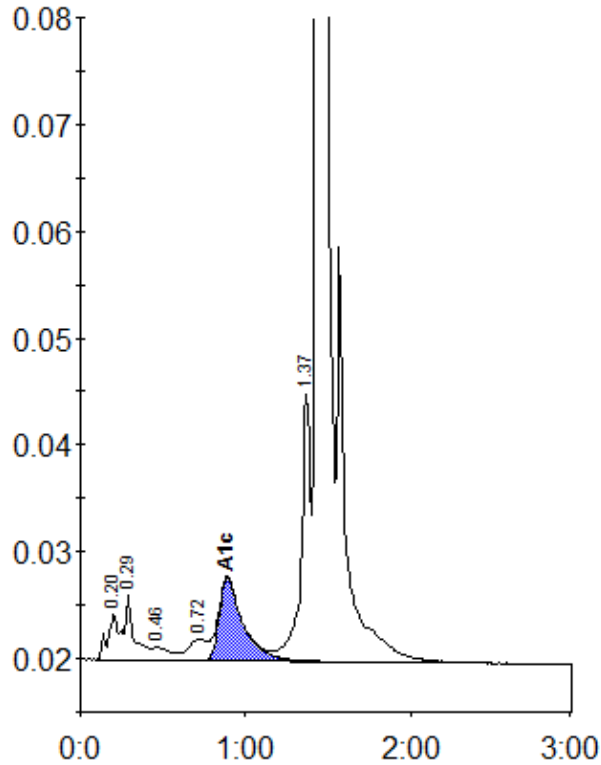
Peak table - ID: 11187318
