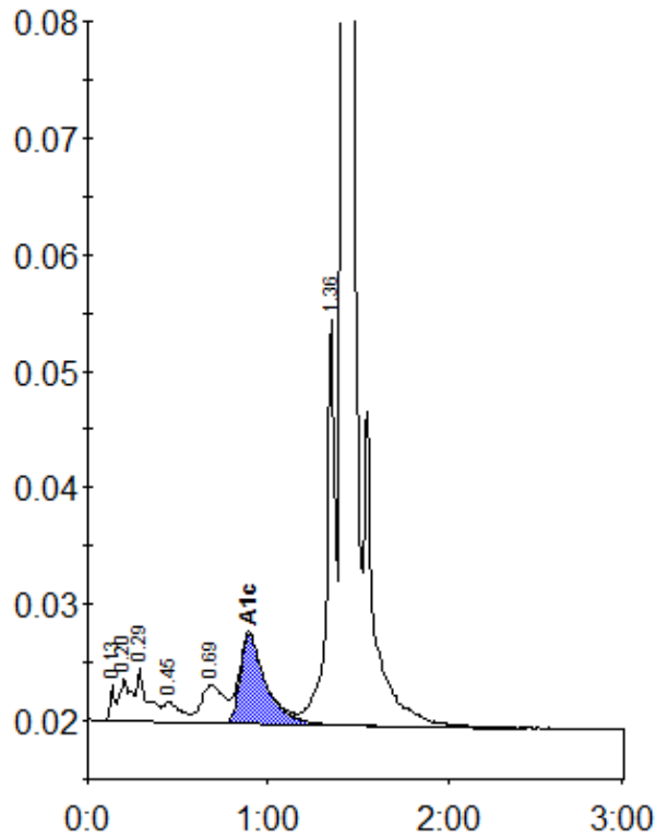
Peak table - ID: 11457477
