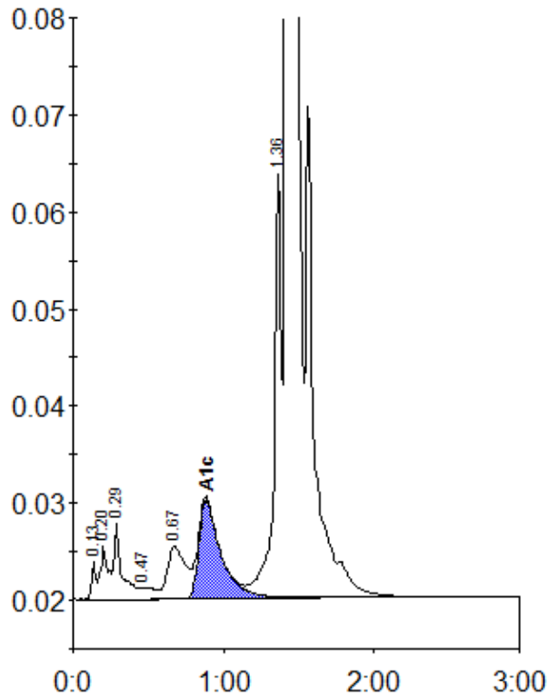
Peak table - ID: 11220658
