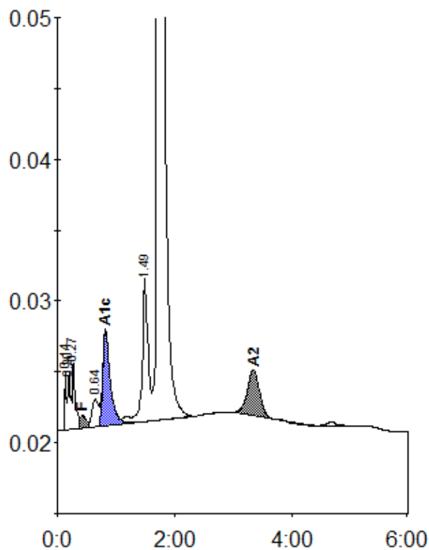
Peak table - ID: 11260048
