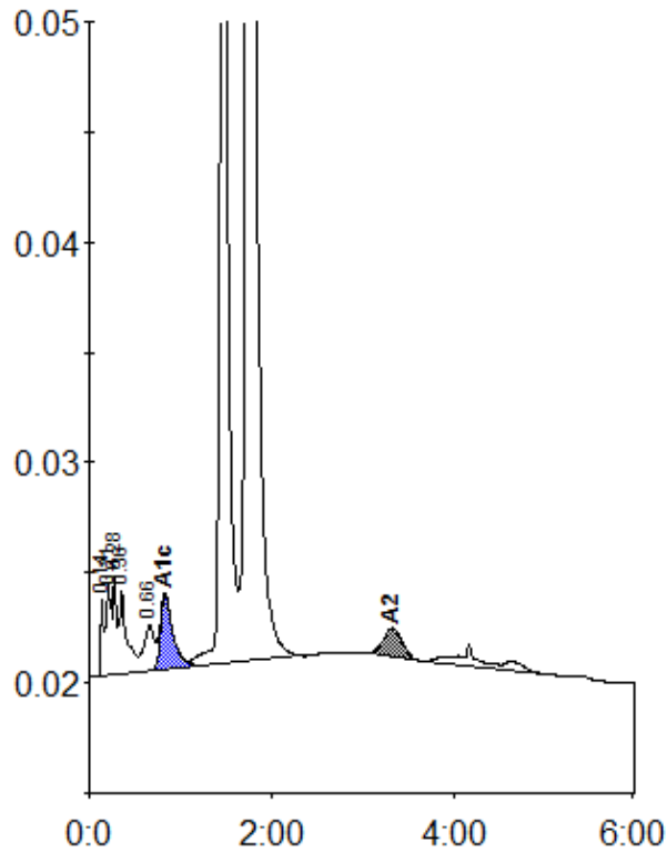
Peak table - ID: 11257865
