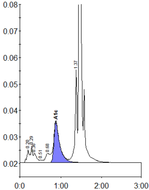
Peak table - ID: 11263110
