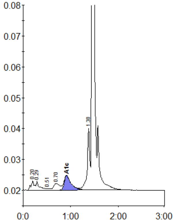
Peak table - ID: 11248273
