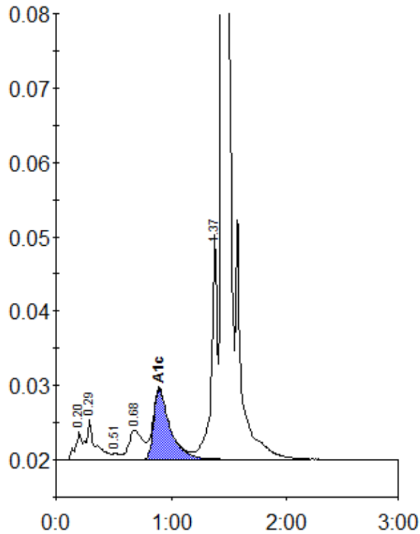
Peak table - ID: 11248281
