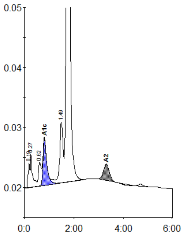
Peak table - ID: 11219264
