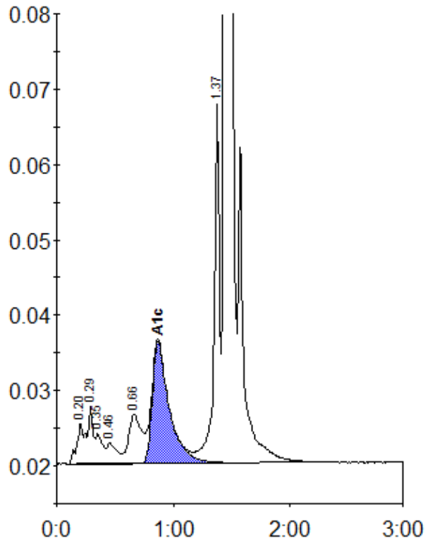
Peak table - ID: 11090802
