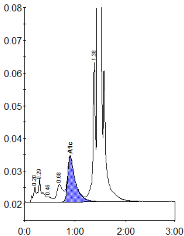
Peak table - ID: 11433402
