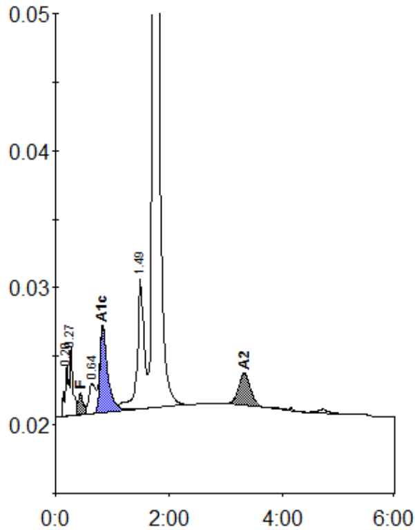
Peak table - ID: 11307299
