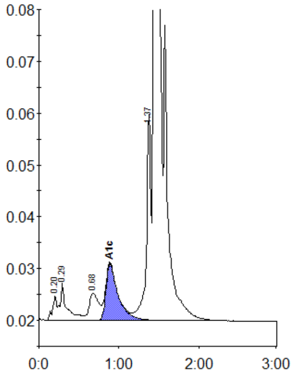
Peak table - ID: 11318624
